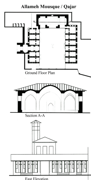
Fig. 26. Plan, Section, and Elevation of the Allameh Mosque, Babol. Source: Registration Dossier in the list of national monuments of Iran, General Directorate of Cultural Heritage, Tourism and Handicrafts of Mazandaran Province.
