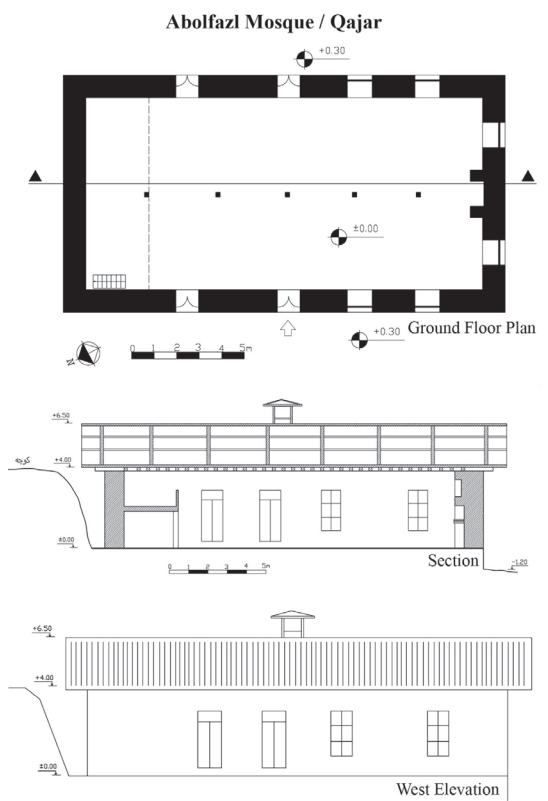
Fig. 33. Plan, Section, and Elevation of Abolfazl Mosque, Aghuz Darreh, Galugah. Source: Registration Dossier in the list of national monuments of Iran, General Directorate of Cultural Heritage, Tourism and Handicrafts of Mazandaran Province.
