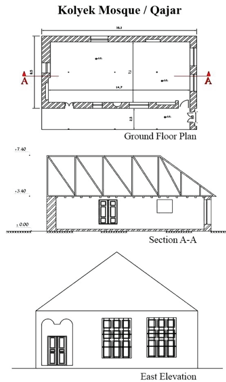
Fig. 40. Plan, Section, and Elevation of Jameh Mosque of Kolyek in Kolyek, Nur. Source: Registration Dossier in the list of national monuments of Iran, General Directorate of Cultural Heritage, Tourism and Handicrafts of Mazandaran Province.
