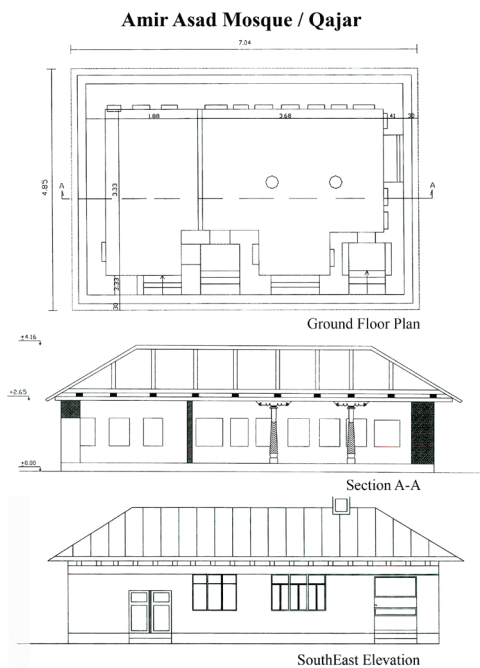
Fig. 31. Plan, Section, and Elevation of Amir As'ad Mosque, Bala-Ashtaj, Tonekabon. Source: Registration Dossier in the list of national monuments of Iran, General Directorate of Cultural Heritage, Tourism and Handicrafts of Mazandaran Province.
