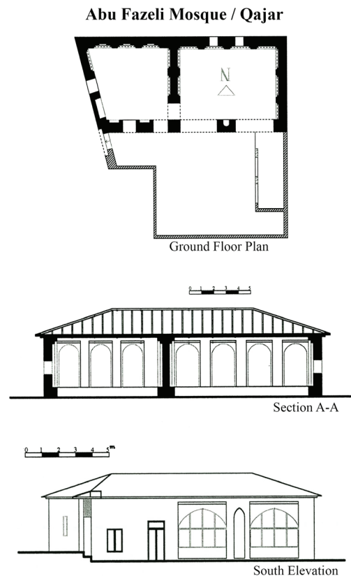
Fig. 34. Plan, Section, and Elevation of Abu Fazeli Mosque, Babol. Source: Registration Dossier in the list of national monuments of Iran, General Directorate of Cultural Heritage, Tourism and Handicrafts of Mazandaran Province.
