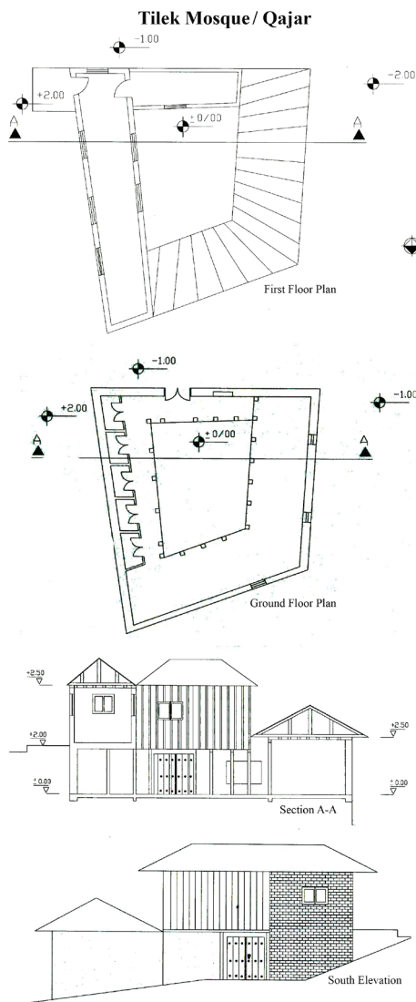
Fig. 53. Plan, Section, and Elevation of Tilek Mosque in Tilek, Sari. Source: Registration Dossier in the list of national monuments of Iran, General Directorate of Cultural Heritage, Tourism and Handicrafts of Mazandaran Province.
