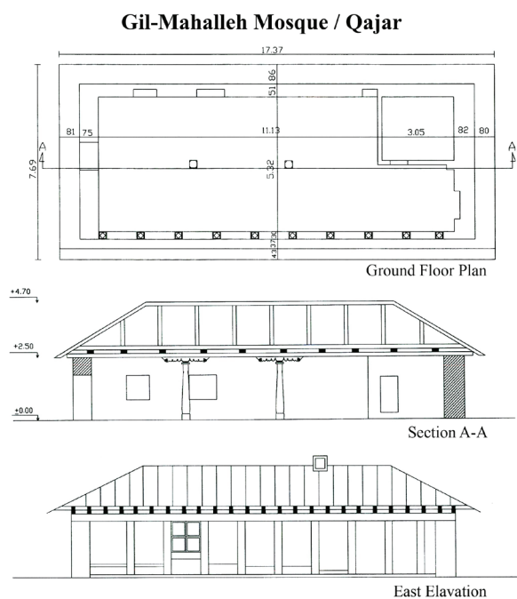
Fig. 32. Plan, Section, and Elevation of Gil-Mahalleh Mosque, Mohammad Abad, Tonekabon. Source: Registration Dossier in the list of national monuments of Iran, General Directorate of Cultural Heritage, Tourism and Handicrafts of Mazandaran Province.
